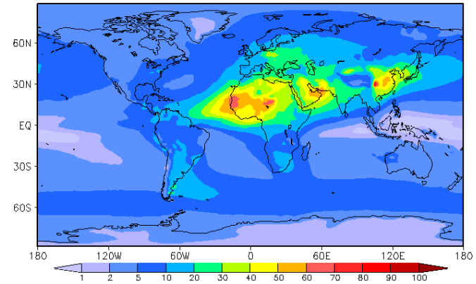
Simulated AOD (2001 – 2006 average) MASINGAR
