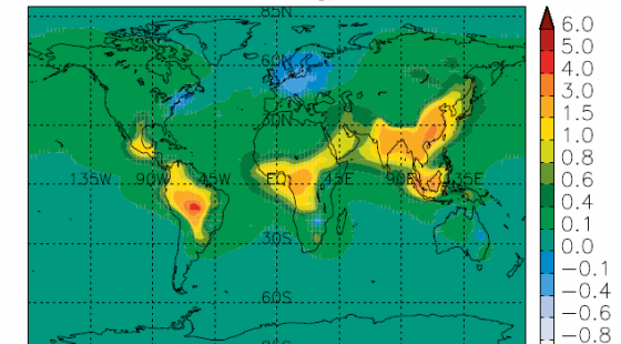
OC ANNUAL mg/m 2 2000–1950
