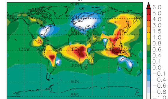
OC ANNUAL mg/m 2 2000–1950
