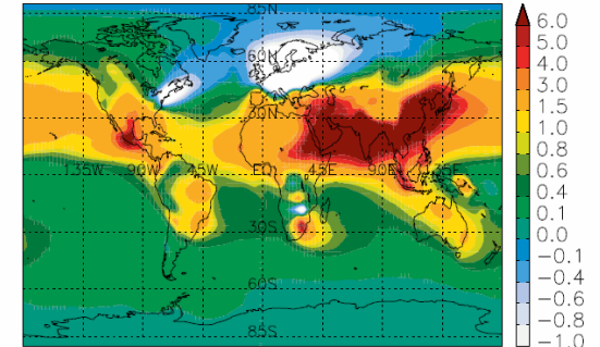
SOAER ANNUAL mg/m 2 2000–1950
