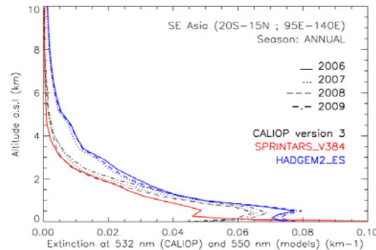
CALIOP version 3 – AeroCom II comparison
