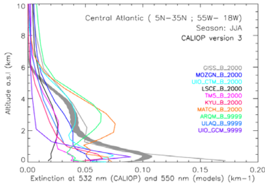
CALIOP version 3 – AeroCom I comparison
