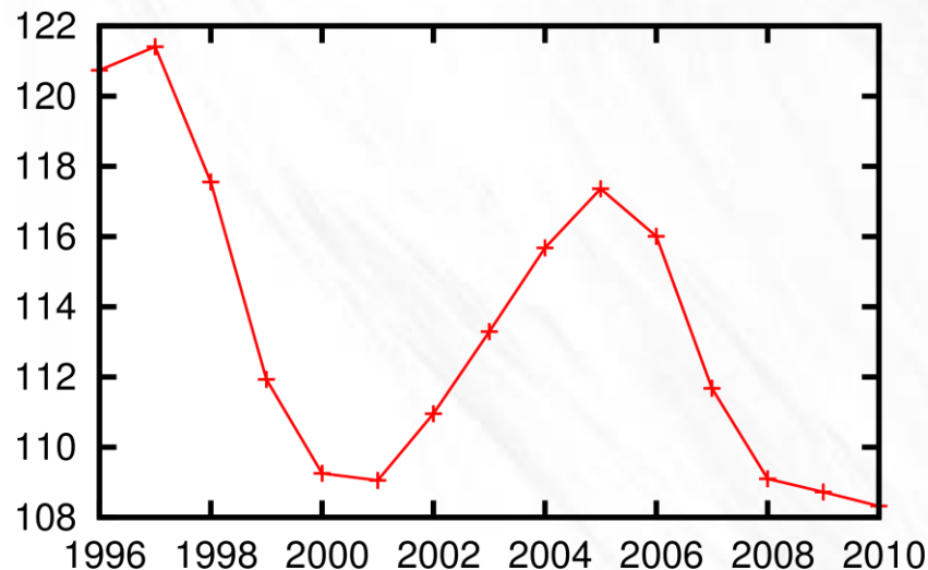
Total SO 2 emissions [Mt] global
