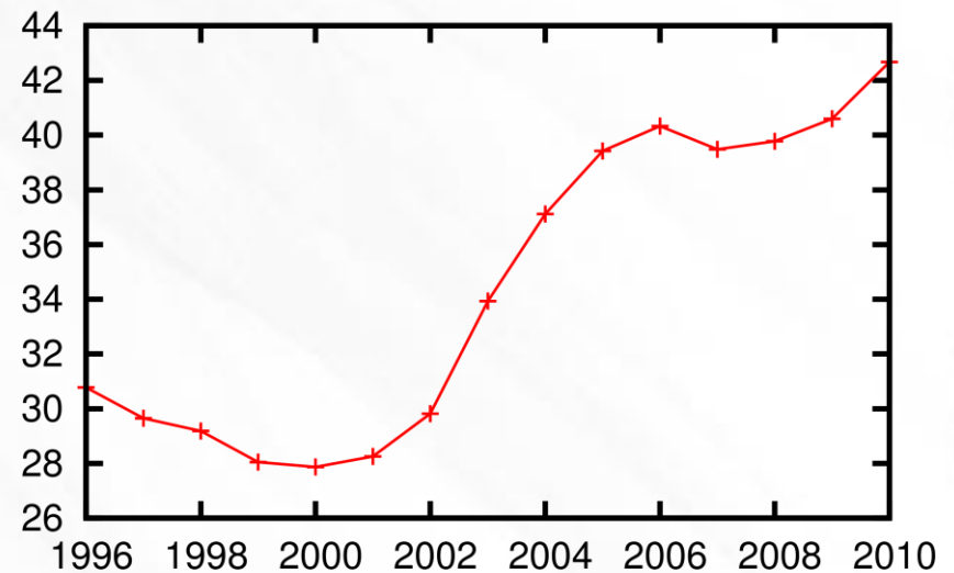
Total SO 2 emissions [Mt] China and India
